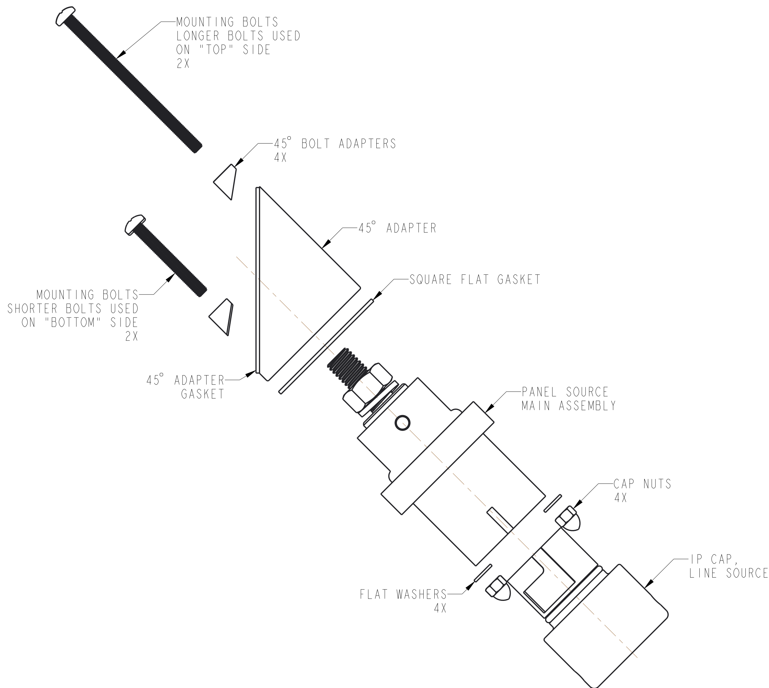
AMPHE-PHASE, PANEL MOUNT SOURCE W/45° ADAPTER - EXPLODED VIEW SCALE 1.00SCALE 1.000
